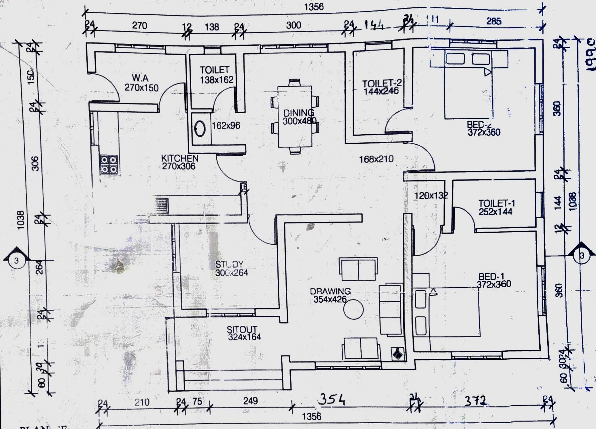
① PLAN OF SCALE 1:100
